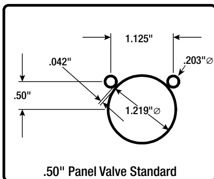
Push - Pull Valve Controls Standard
