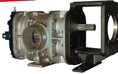
Model H Hydraulic Mount
