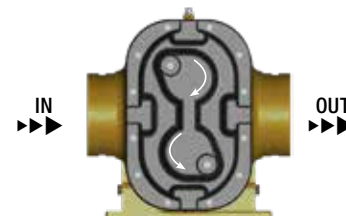
Timing Gear Cover Rear of Pump
